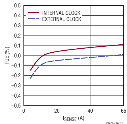
Energy Measurement Total Unadjusted Error vs Current, VP – VM = 12V
